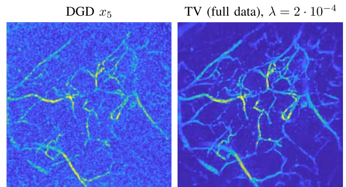
Fig. 4. Reconstruction from real measurement data of a human palm, without adjustments of the training data. The images shown are top-down maximum intensity projections. Left: Result of the DGD trained on images without added background. Right: TV reconstruction as reference from fully sampled data.
